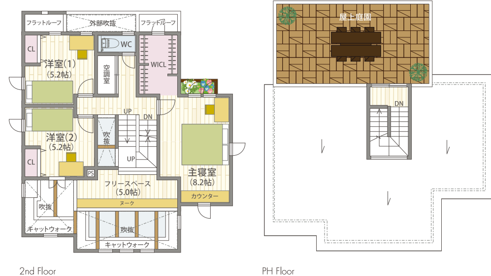
2nd Floor
