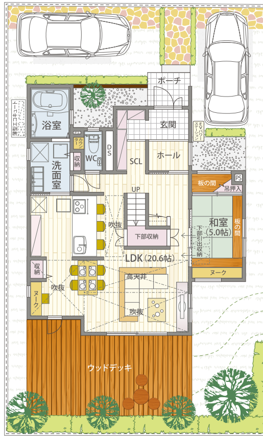
1st Floor
